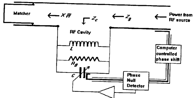
Figure 2. Cavity and feed circuit model
