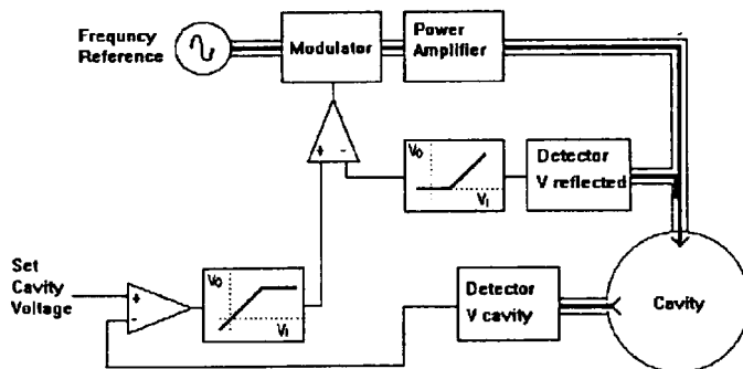
Figure 4. Cavity voltage control loop
