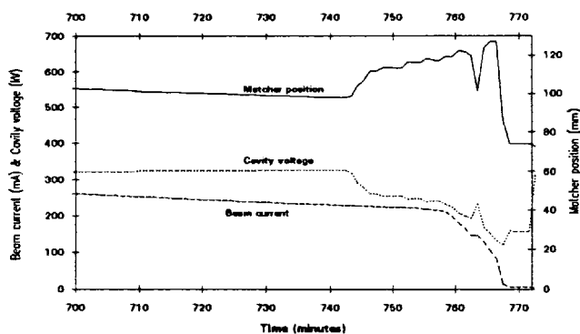
Figure 3. Matcher movement in response to a change in cavity voltage and stored current at full energy
