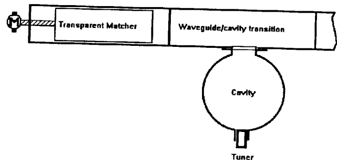
Figure 1. Waveguide feed and cavity
